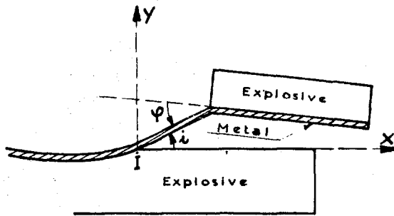
Fig 1 - Experimental arrangement
